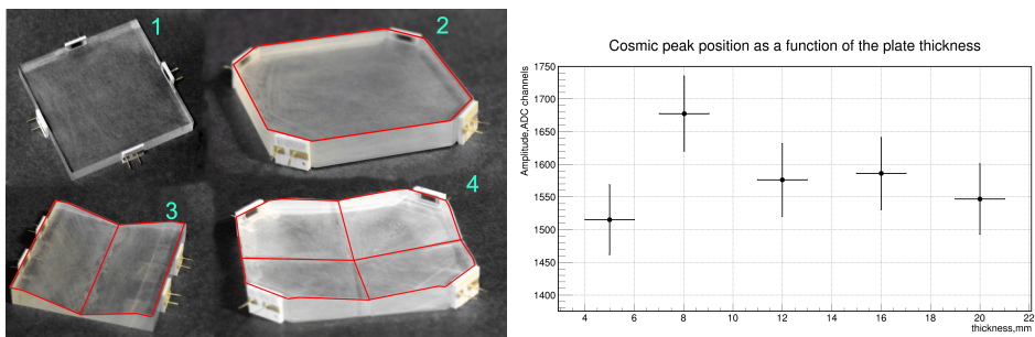
Figure 1. PMMA plates of different shapes/types (left); position of the cosmic peak for the PMMA plates of type 4 with different thicknesses (right).
